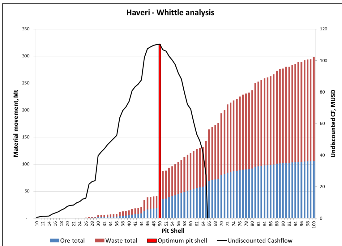
Figure ES 1: Pit optimisation results (Source: SRK, 2014)
