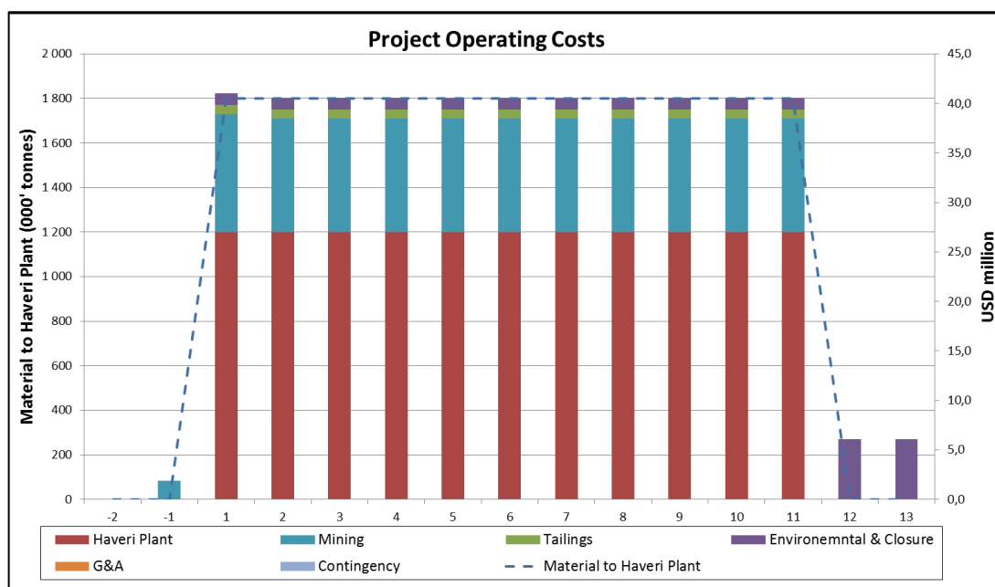
Figure 21-1: Summary of operating costs over the life of mine (Source:SRK, 2014)
