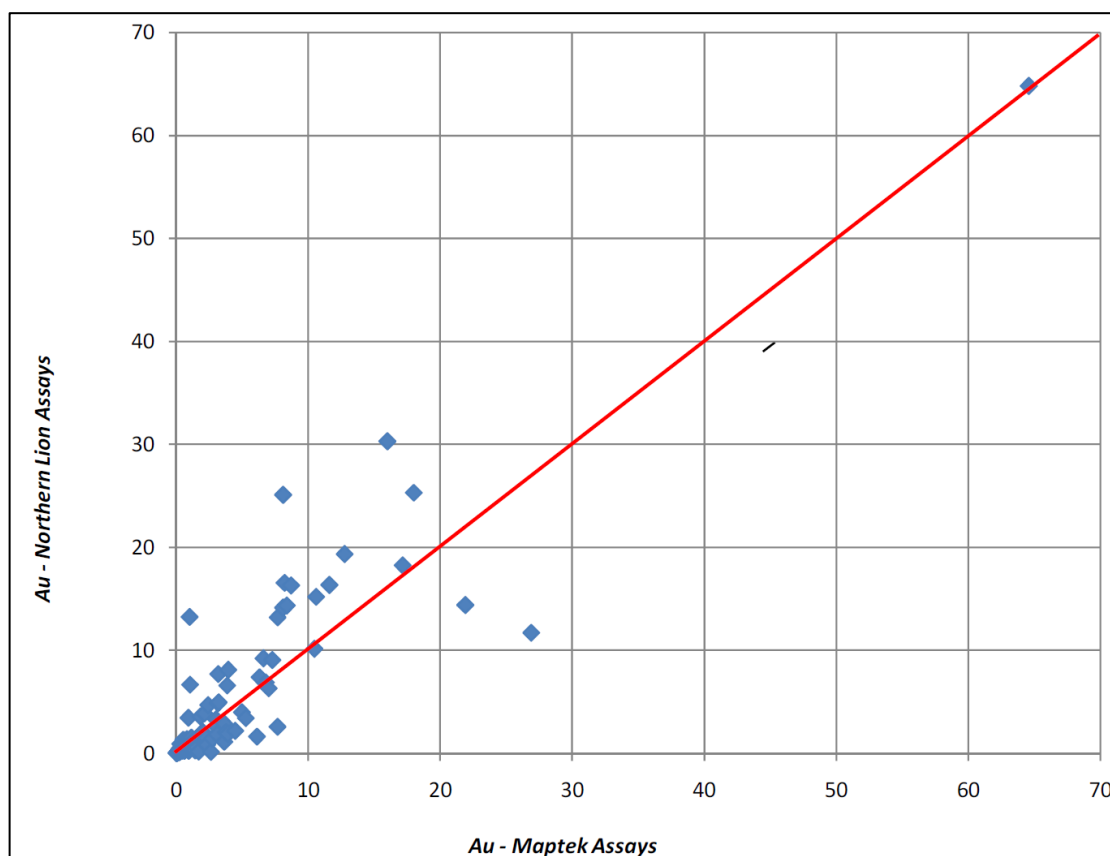
Figure 12-1: Maptek check Au assays vs original assays (Source: Reed, 2008)
