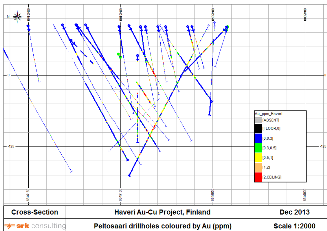
Figure 6-14: Cross-section through Peltosaari mineralisation
